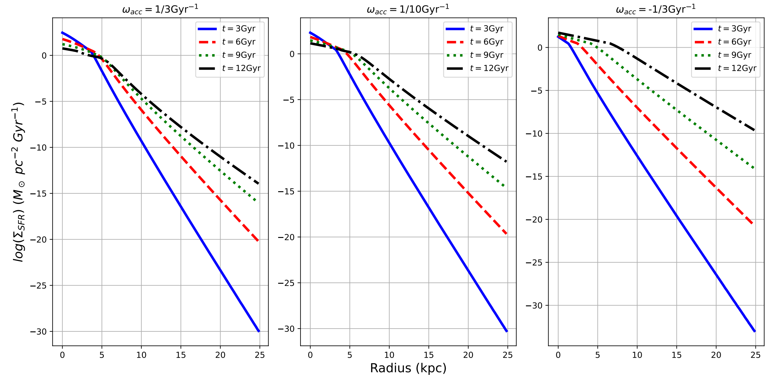
\Sigma_{SFR} vs r for different t and t_{acc}
